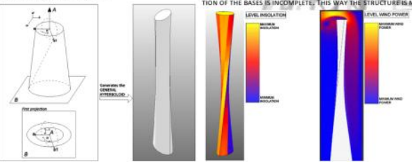
FIG. 11. GEOMETRY OF THE CANTON TOWER IN FIRST PROJECTION. FIG. 12. INSOLATION ANALYSIS AND WIND SIMULATION FOR THE GEOMETRY OF CANTON TOWER.
