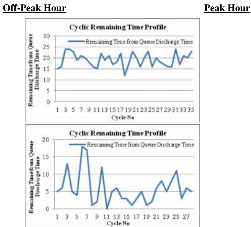
Figure 3 Cyclic Remaining Time Profiles for Cinar Approach
