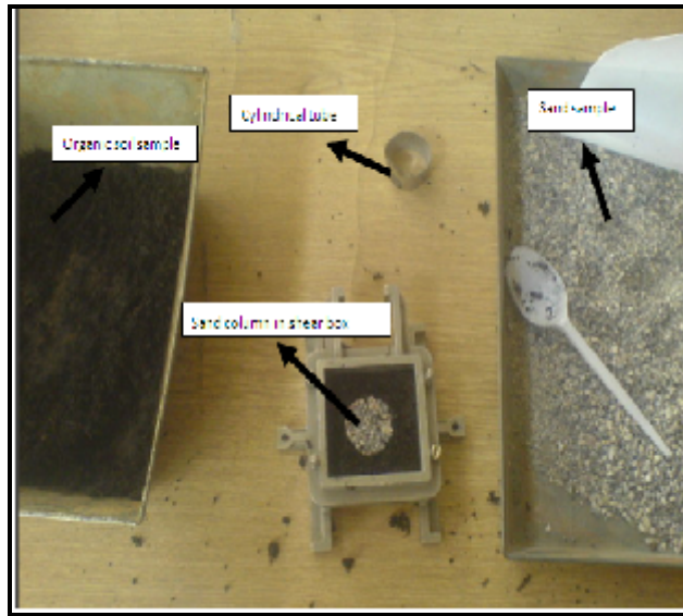
Figure 4 Test samples and shear test apparatus
