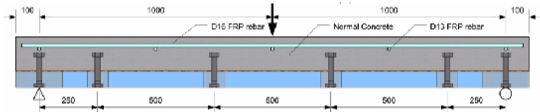
Figure 2 GFRP Deck
